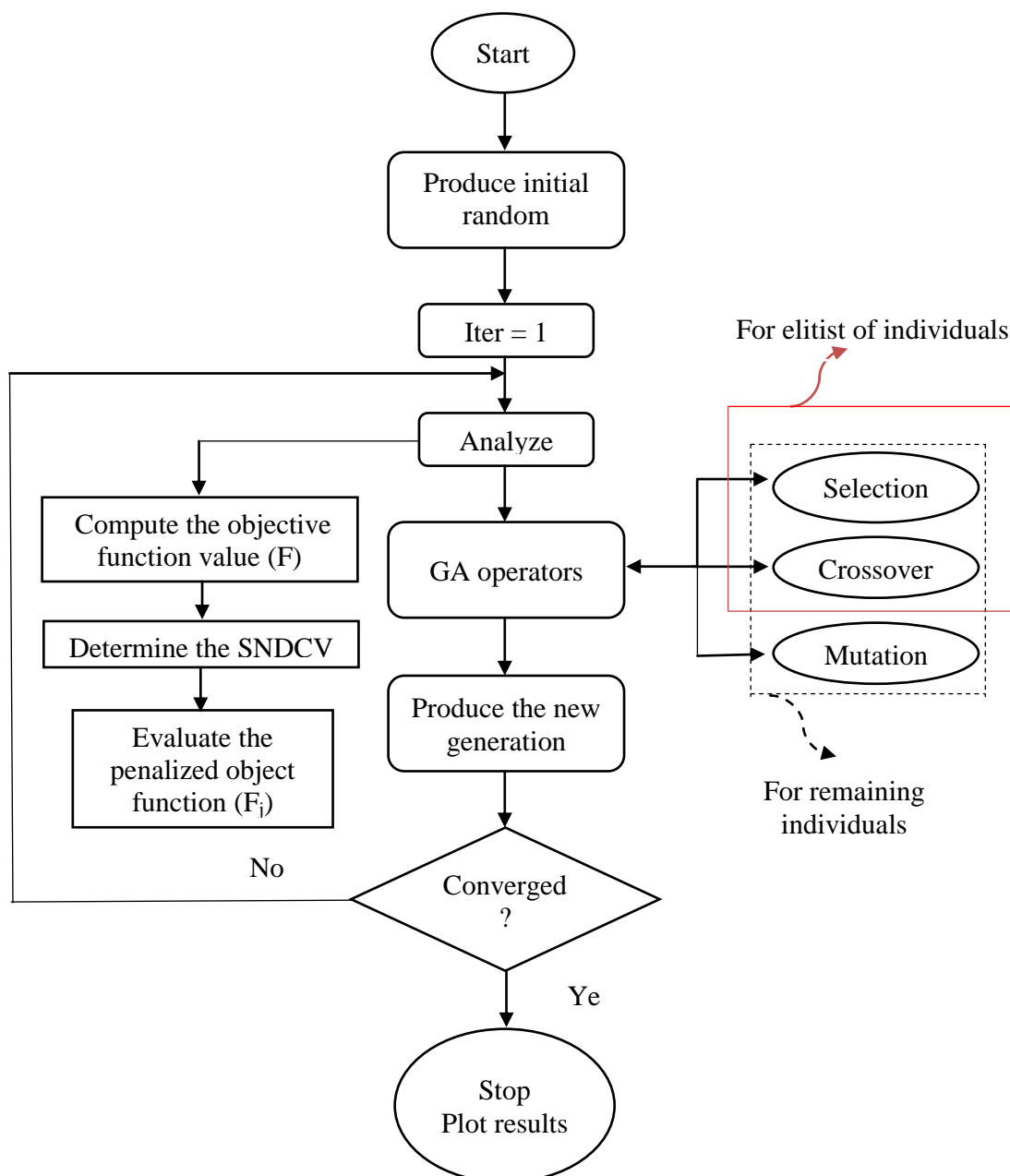
Figure 1. Flowchart of the proposed GA method
