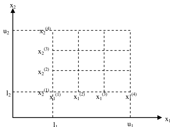
Figure 1. Grid with p_i=4 [26]
