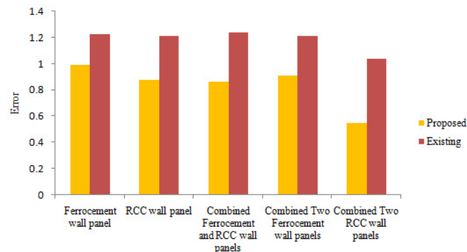
Figure 7. Comparison graph
