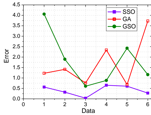
Figure 6. Error graph for combined two RCC wall panels
