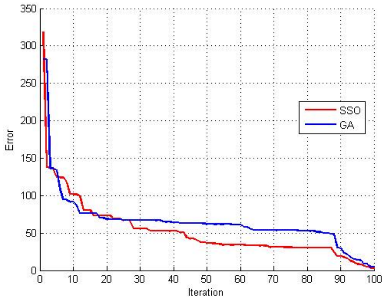
Figure 1. Convergence graph
