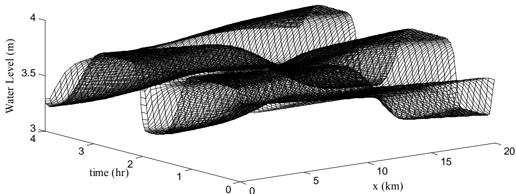
Figure 4. A 3D view of water level fluctuations in the whole channel over simulation time when no control (dashed line in Figure 2) is imposed at upstream end ( f=2396.33 \text{ m} )
