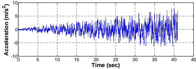
Figure 8. ETA40d01 acceleration function
