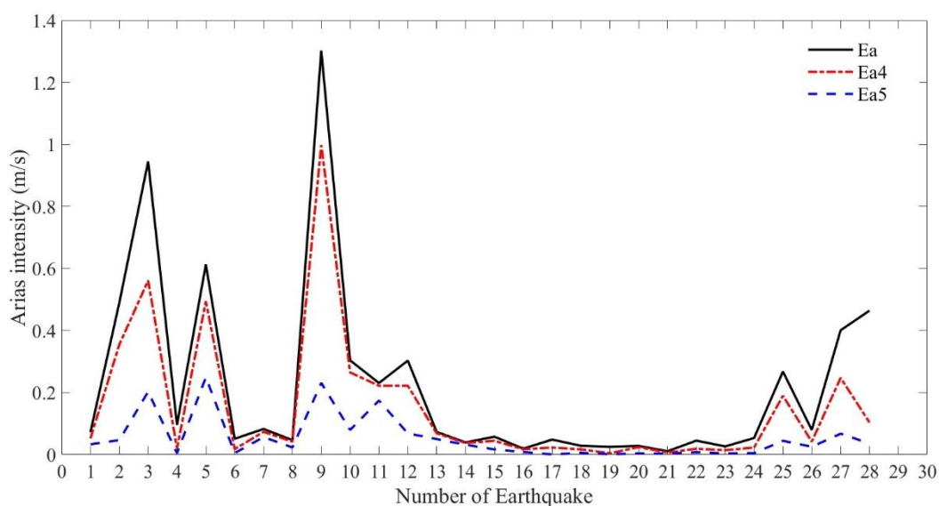
Figure 6. The Arias intensity for Ea , Ea4 and Ea5
