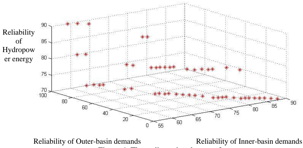
Figure 4. Three-dimensional pareto fronts
