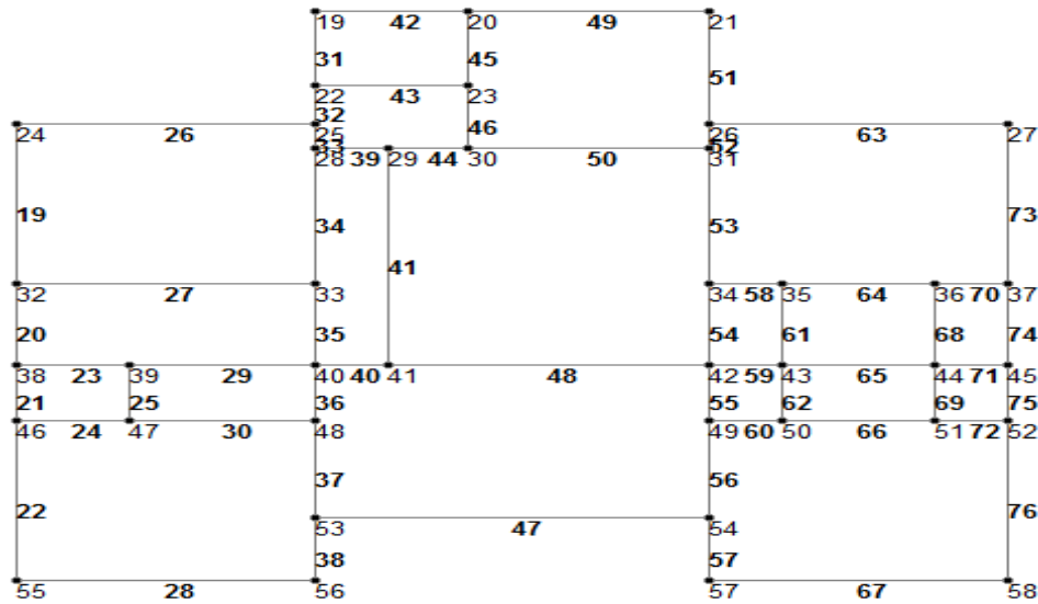
Figure 3. Plinth with node and member
