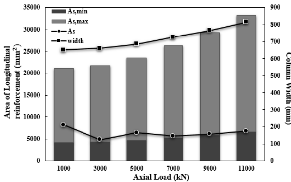
Figure 7a. Variation of longitudinal rebar section and optimal column dimension with respect to variation of axial load in constant bending moment of 1000\text{ kN.m}
