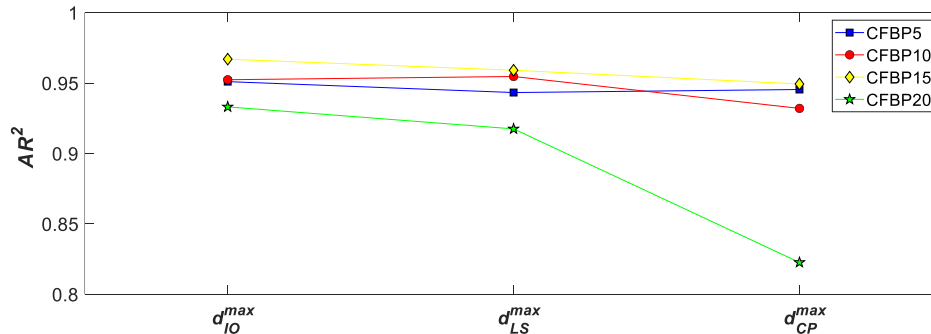
Figure 12: AR^2 of predicted inter-story drift ratios for the 6-story frame
