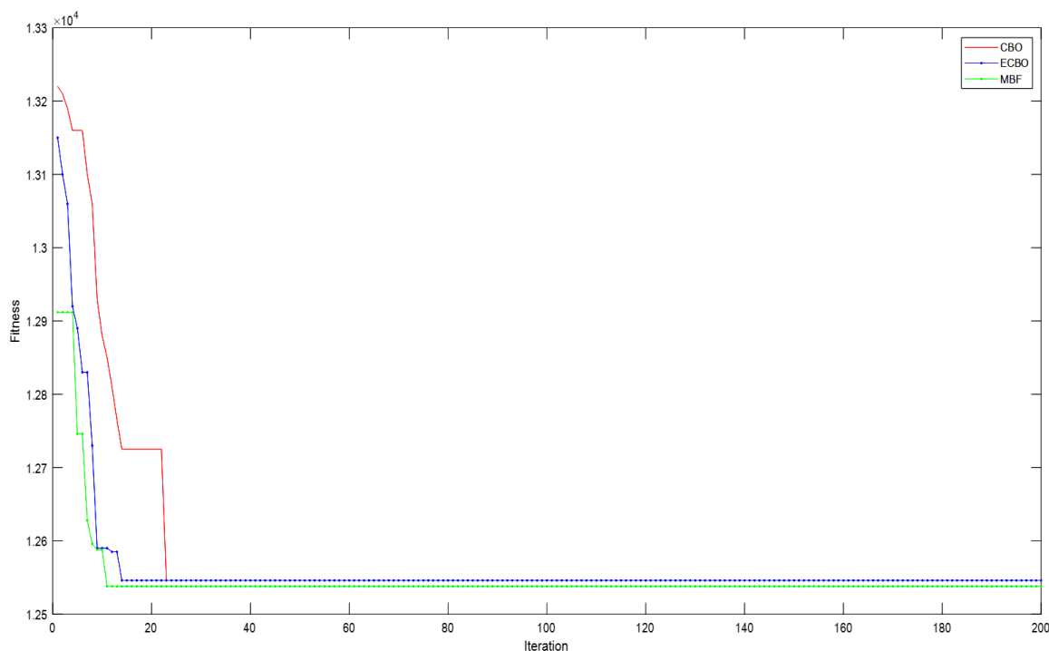
Figure 2: Convergence history of the MBF algorithm
