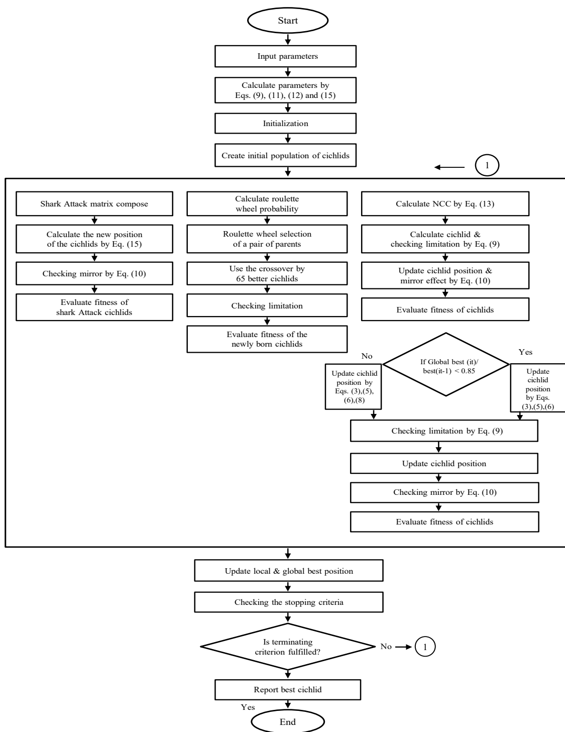
Figure 1: Flowchart of the MBF Algorithm [23]
