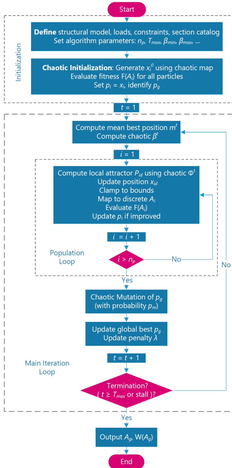
Figure 2: Flowchart of proposed CQPSO algorithm
